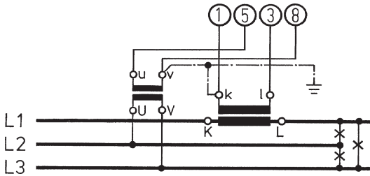
3-Pahse 3-Wire, Balanced Load
