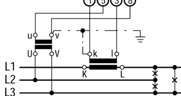
3-Phase 3-Wire, Balanced Load Active & Reactive Power
